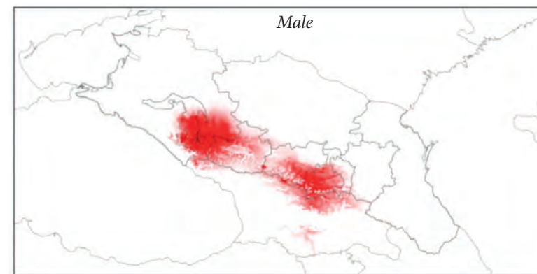
Fig. 10. Potential ecological corridors between leopard release sites and developing groups. The modeling was carried out on the base of gps-coordinates obtained from collars released leopards were tagged with.
