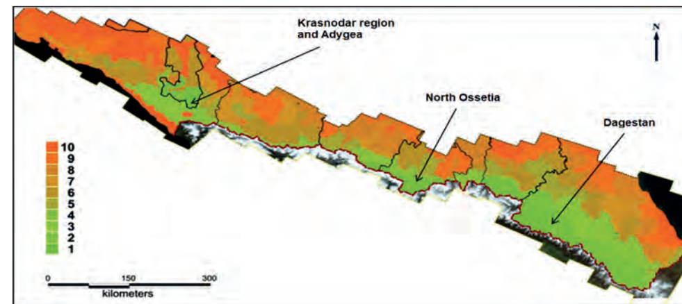
Fig. 2. The potential range of the Persian leopard in the Russian part of the Caucasus. Map is based on remote sensing data of the Earth. An anthropogenic pressure map for the leopard's potential habitat in the Russian Caucasus (points ranging from 1 to 10) reflect the degree of anthropogenic impact and intensity, optimal habitats are areas painted in bright green.
